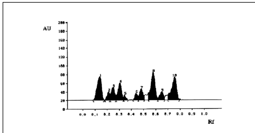
Fig. 2: HPTLC chromatogram of Tinospora cordifolia test sample (Rf = 0.58).
