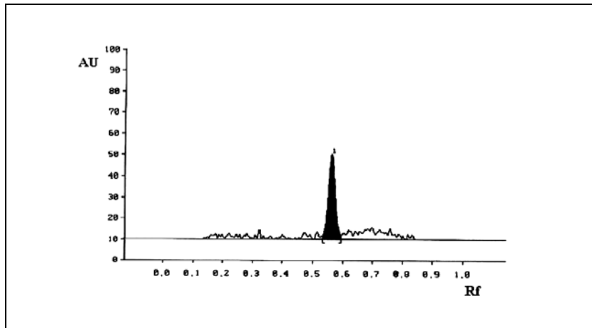
Fig. 1: HPTLC chromatogram of standard Tinosporaside (Rf = 0.58).
