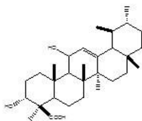
3-O-11-hydroxy-beta-boswellic acid
