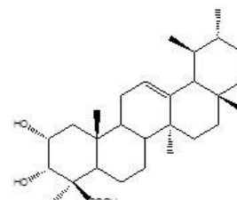
2, 3-dihydroxy-urs-12-ene-24-oic acid
